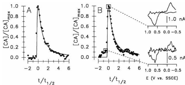
FIGURE 3 Normalized spikes detected by cyclic voltammetry. Each data point is the concentration determined from a single cyclic voltammogram recorded at the time indicated, and the solid lines are the curves obtained by digital simulation of instantaneous point-source release and diffusional transport to the electrode. (A) Spike recorded with a 5- \mu m cell-electrode spacing. Spike characteristics: [\text{CA}]_{\text{max}} = 22.4 \mu\text{M} ; t_{1/2} = 62 \text{ ms} ; R = 0.978 . (B) Spike recorded with a 1- \mu m cell-electrode spacing. Spike characteristics: [\text{CA}]_{\text{max}} = 40.8 \mu\text{M} ; t_{1/2} = 177 \text{ ms} ; R = 0.975 . Background-subtracted voltammograms were obtained by averaging the three voltammograms obtained at the times indicated by the points enclosed by the associated boxes.
