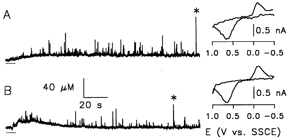
FIGURE 2 Cyclic voltammetric response measured at the catechol oxidation wave (750 mV vs. SSCE) in successive scans from individual cells in response to 20 \mu M digitonin (exposure for 8 s) in the presence of 2 mM \text{Ca}^{2+} . The concentration axis was obtained from electrode calibration. (A) 1- \mu m cell-electrode spacing. (B) 5- \mu m cell-electrode spacing. In each trace, the stimulus application is shown by the horizontal bar below the trace. The background-subtracted voltammograms were obtained from the points designated by asterisks.
